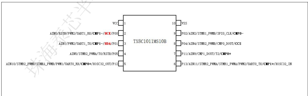
Figure 1-4 Pin of TX8C1011MS10B
