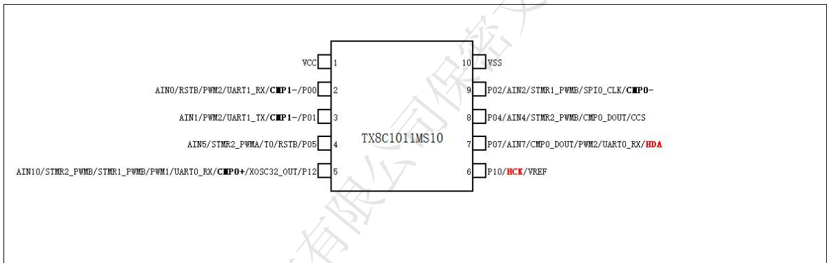
Figure 1-3 Pin of TX8C1011MS10
