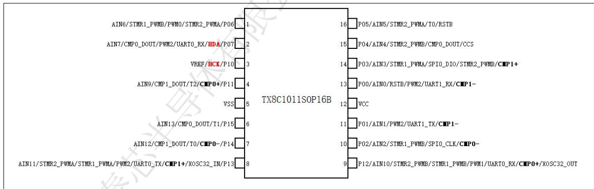
Figure 1-7 Pin of TX8C1011S016B
