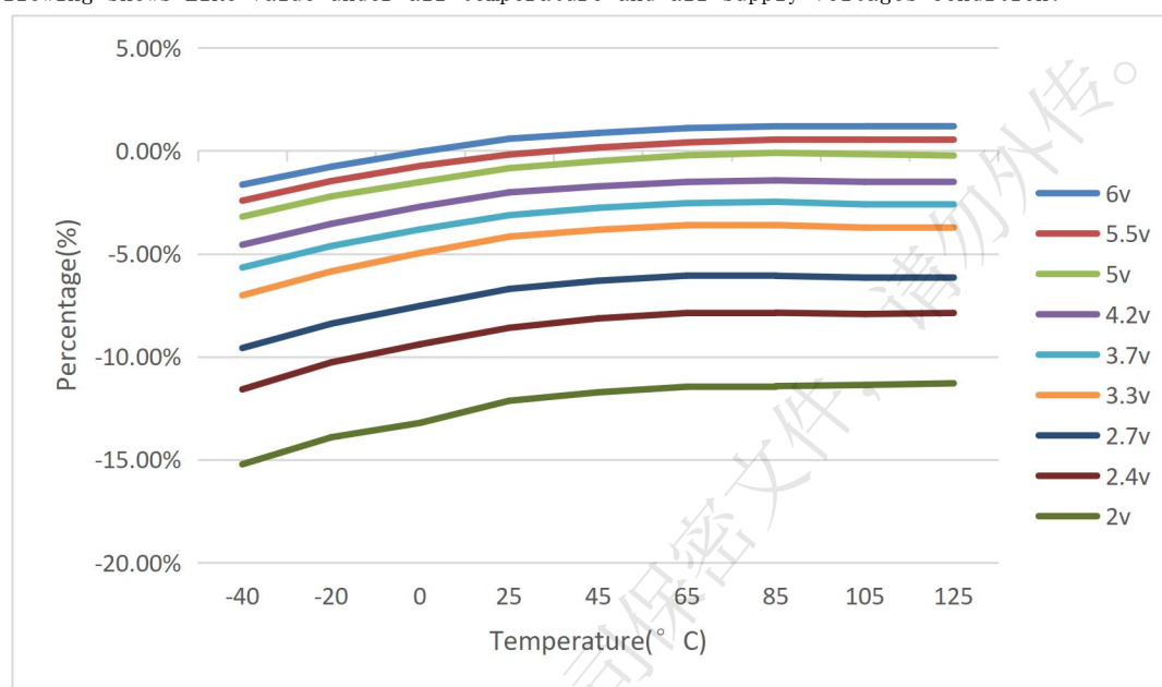
Figure 2-4 LIRC deviation under all voltage and all temperature
