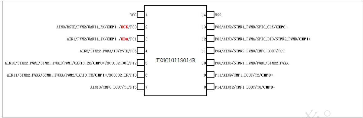
Figure 1-5 Pin of TX8C1011S014B
