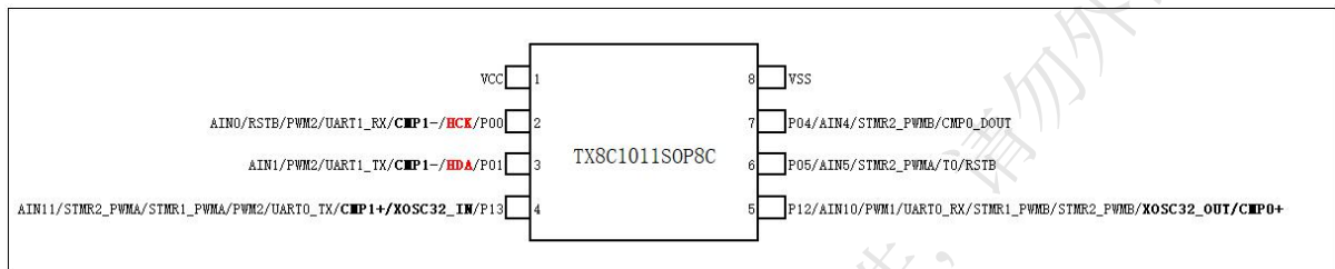
Figure 1-2 Pin of TX8C1011S08C
