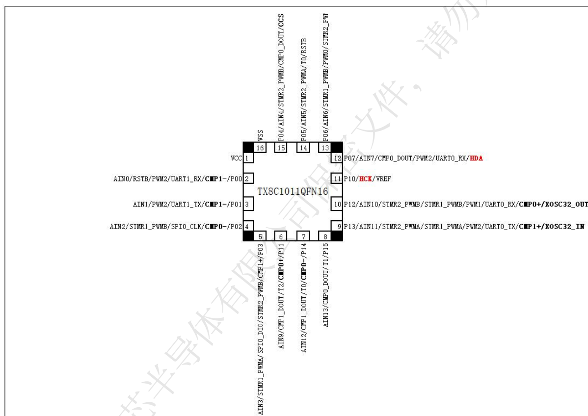
Figure 1-9 Pin of TX8C1011QFN16
