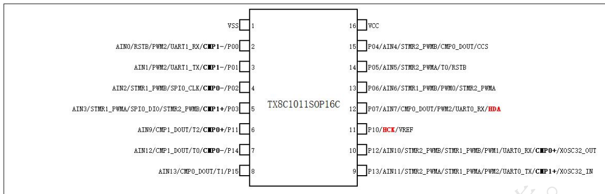
Figure 1-8 Pin of TX8C1011S0P16C
