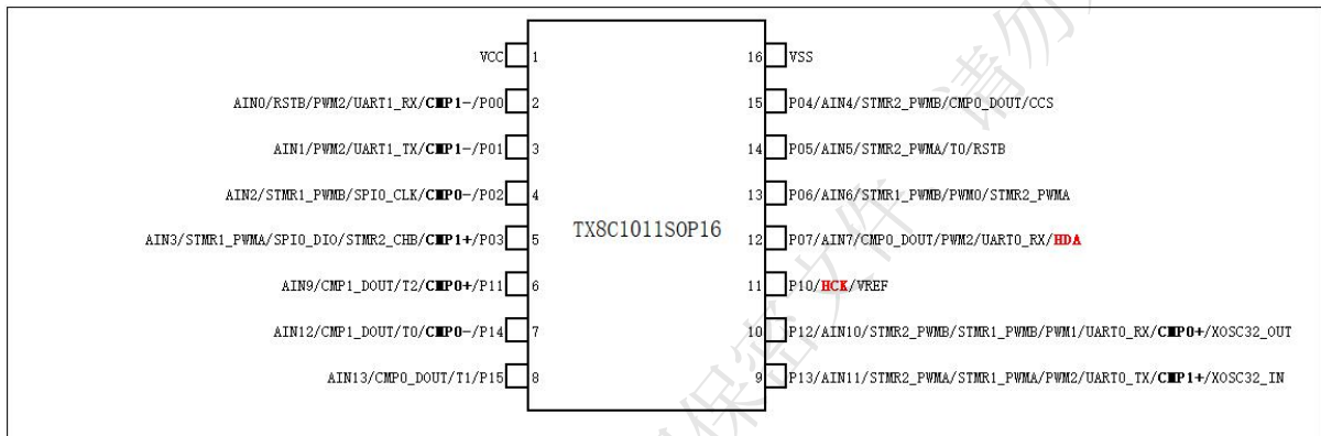
Figure 1-6 Pin of TX8C1011S016
